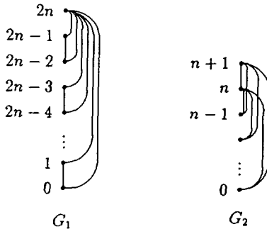
FIG. 2. Vertices of a star exploded into edges.
