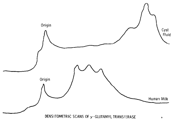
Fig. 1. Densitometric scans of electrophoresis \gamma -glutamyl transferases of human breast cyst fluid and colostrum milk. 0.3 \mu\text{l} samples were electrophoresed at 250 V and 5–10 ma for 45 min at pH 8.8 on Sepharose III cellulose acetate strips in a Beckman Microzone system. The \gamma -glutamyl transferase was located by incubating the strips in 1.25 mM \gamma -glutamyl- \beta -naphthylamide and 2 mM glycylglycine at pH 8.2 for 30 min at 37^\circ\text{C} followed by a 5 min incubation in a solution of Diazo Blue B, 5 mg per ml in acetic acid and water (15:85).
