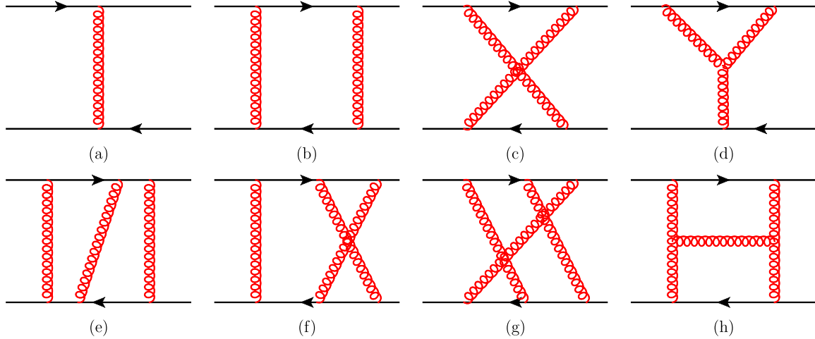
Fig. 1. Sample diagrams contributing to V_{ij}^{[c]} at tree-level (a), one-loop (b)–(d) and two-loop order (e)–(h). The straight lines correspond to quarks or gluinos, respectively, and the curly lines represent gluons.
