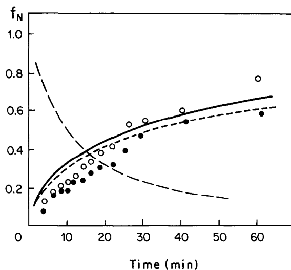
Fig.2. Time dependence of fraction of nativity f_N in the course of CA B refolding from the molten-globule state (I \rightarrow N transition from 1.97 M to 0.97 M Gu-HCl) monitored by ellipticity at 270 nm (----) and esterase activity (o). Time dependences of these values at U \rightarrow N transition (— and o, respectively) are reproduced from fig.1 for comparison. Curve (—) shows the kinetics of the N \rightarrow I (0.97 M \rightarrow 1.97 M Gu-HCl) transition.
