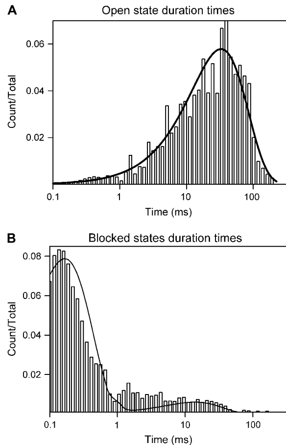
FIGURE 4 Example of the distributions of the duration of the open state ( A ) and blocked states ( B ) of G3139-induced rapid flickering of a single VDAC channel with 5 \mu\text{M} G3139 added to the cis side and -40 mV applied voltage.
