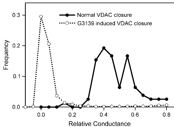
FIGURE 2 Comparison of the distribution of relative conductance of normal VDAC closure and G3139-induced VDAC closure. G3139 (10 \mu\text{M} ) was added to the same side as the VDAC addition.
