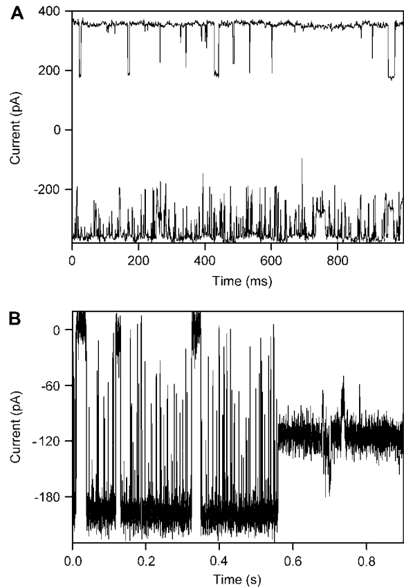
FIGURE 3 (A) Asymmetric flickering of VDAC induced by 40 \mu\text{M} G3139 present on both sides of the membrane. A voltage of -50 mV was applied to the cis side (lower trace) and to the trans side (upper trace). Two VDAC channels were present in the membrane. Recordings were made at 1 ms per point with 2-kHz filtering. (B) No flickering occurs when VDAC enters a normal closed state. This is a typical experiment of a single VDAC with flickering induced by 10 \mu\text{M} G3139 on the cis side. The applied voltage was -50 mV.
