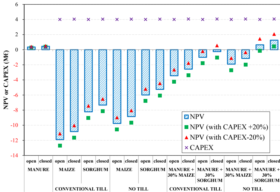
Fig. 3. Net Present Values of the systems considered. The CAPEX is reported to facilitate the evaluation of the performances.
