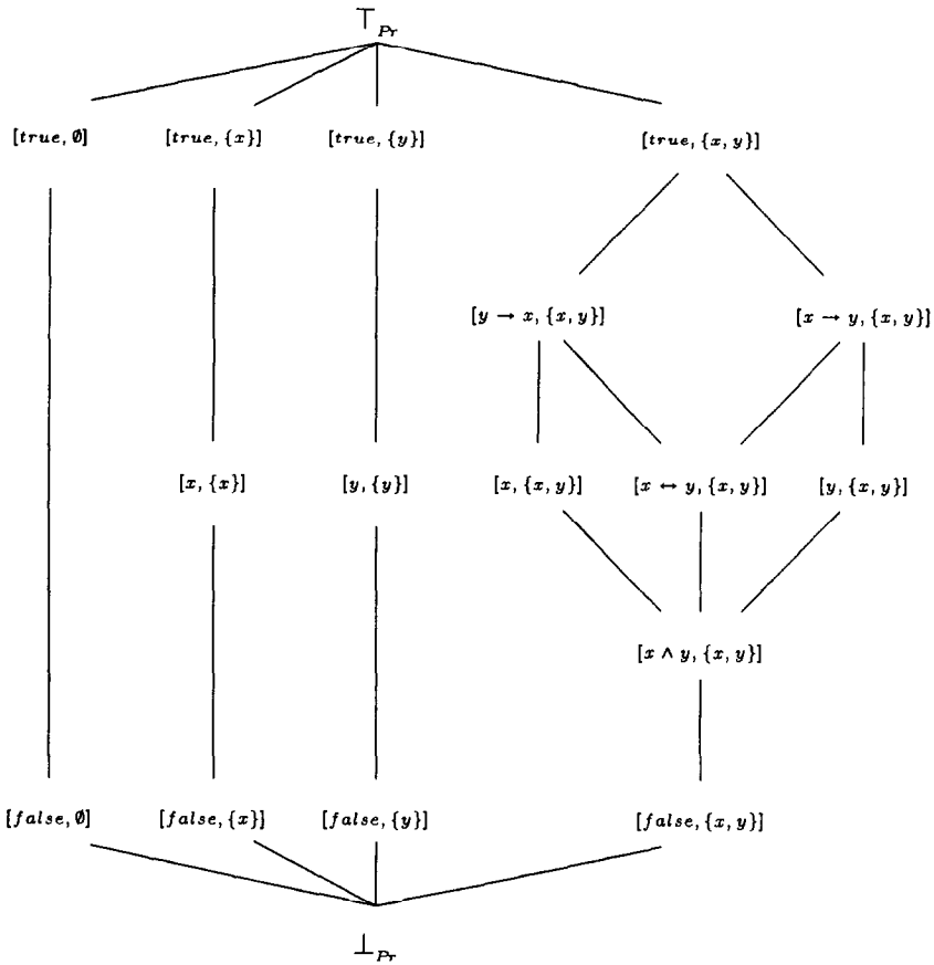
Fig. 5. The quotient \mathcal{Q}_{GR}(\text{Sharing}) for V = \{x, y\} .
