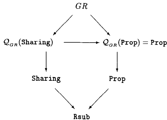
Fig. 6. Domain abstractions.
