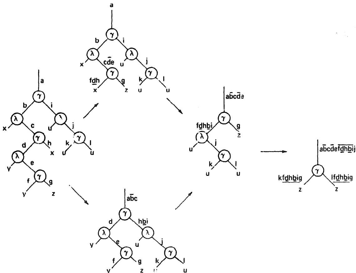
Fig. 1. Reductions from ((\lambda x \cdot (\lambda y \cdot (y'z^a)^{t'x^h})^c)^\beta (\lambda u \cdot (u^t u^t)^t))^\alpha .
