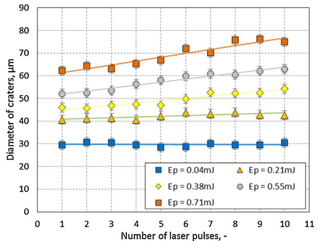
Fig. 4. Diameter of craters as a function of number of laser pulses for different pulse energies. Solid lines are trend lines.
