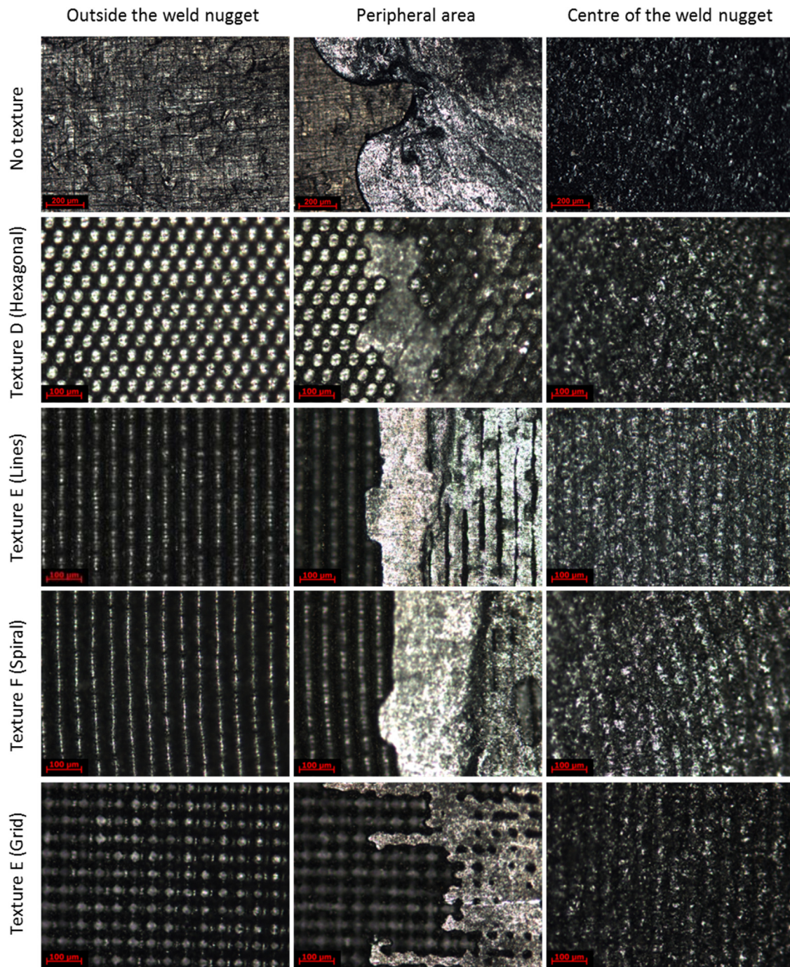
Fig. 12. Micrographs showing the fracture surface on the steel side after tensile-shear testing. The samples were produced using PD = 20.1 \text{ MW/m}^2 and t_1 = 3 \text{ s} .
