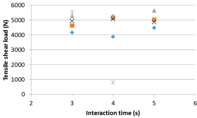
Fig. 10. Tensile shear load as a function of the interaction time for different laser-textured and untextured samples. The results were obtained with PD = 20.1 \text{ MW/m}^2 .
