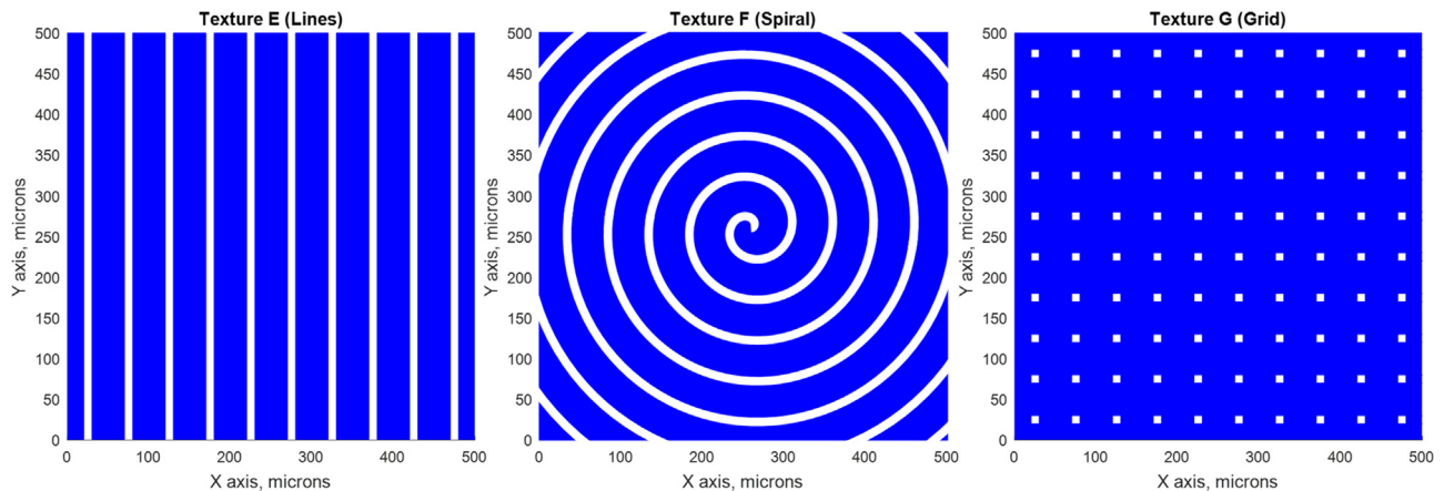
Fig. 9. Schematic of laser-generated textures comprising parallel troughs (Texture E), spiral pattern (Texture F) and a grid of troughs (Texture G). White area represents the contact area between the aluminium and the steel surface, whereas blue area represent the laser-textured area. (For interpretation of the references to colour in this figure legend, the reader is referred to the web version of this article.).
