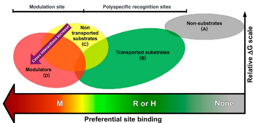
Fig. 3. Classification scheme for P-gp substrates. Reprinted with permission from [78]. Copyright 2013 American Chemical Society.
