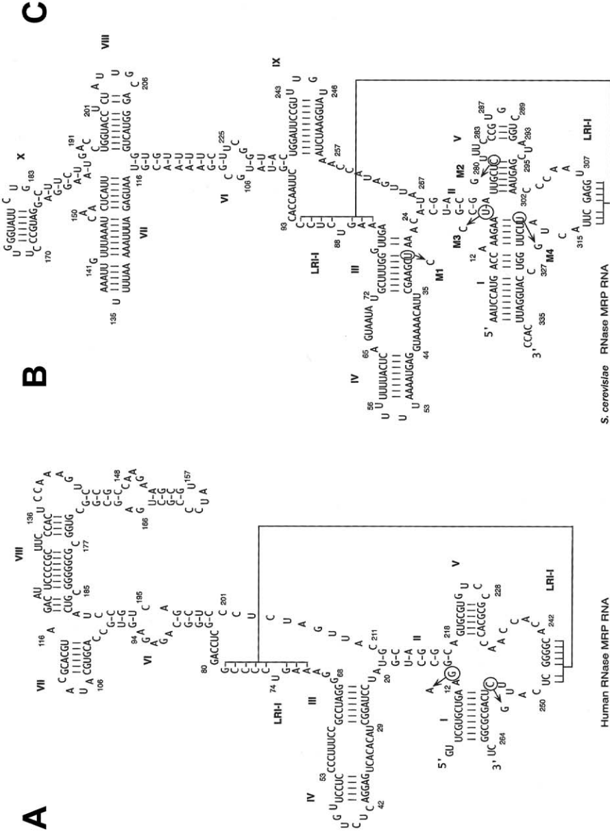
Figure 5 Scheme of the two-dimensional structure of RMRP and nme1 RNA and the results of nme1 mutant analysis in S. cerevisiae . A, Predicted two-dimensional structure of human RMRP RNA, showing the position of the anaerobic dysplasia mutations +14G→A and +254C→G. B, Predicted two-dimensional structure (Shadel et al. 2000) of yeast nme1 RNA, showing positions considered equivalent by sequence alignment (M3 = +254C → G) or structural alignment (M3 = +14G → A and M4 = +254C → G). C, Reduced colony growth and metabolic activity in M1–M4 colonies grown on YPD and YPG plates at 30°C and 34°C, as compared with wild-type colonies that show red color due to an ade2 marker. Because of a mutation in the ade2 gene, adenine biosynthesis is impaired, which leads to the accumulation of an oxidized ( red ) precursor in yeast with normal metabolic activity.
