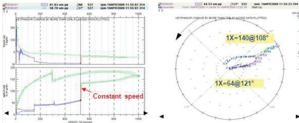
Fig. 6. Direct and 1X Bode plots with 1X polar plots for NDE generator bearings during run up/coast down with a step at 500 rpm showing vibration increase and phase change
