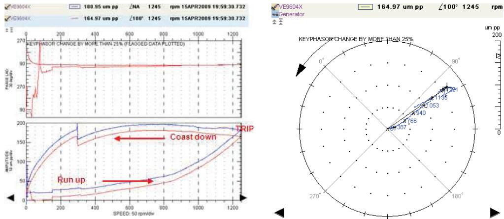
Fig. 3. Direct and 1X Bode plots with 1X polar plot for NDE generator bearings during run up and coast down after a trip because of high vibrations
