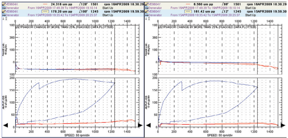
Fig. 9. 1X Bode plots showing the difference in vibration level before (in blue) and after (in red) the issue
