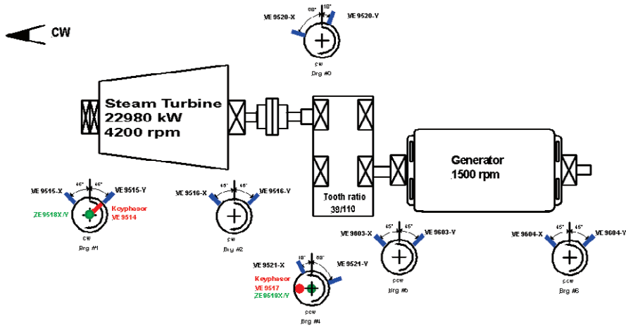
Fig. 1. Machine train layout
