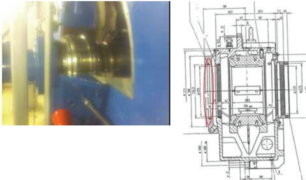
Fig. 10. Picture and drawing showing seals details on generator bearings (air cooled generator)
