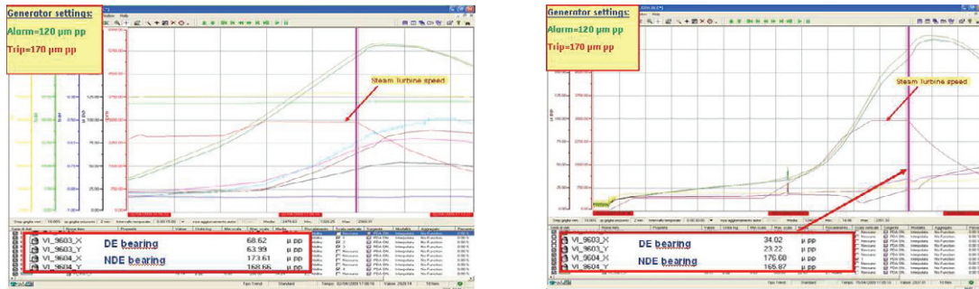
Fig. 2. Customer data showing high vibrations on generator bearings while trying to reach nominal speed. Data show two attempts to reach synchronization speed within two weeks
