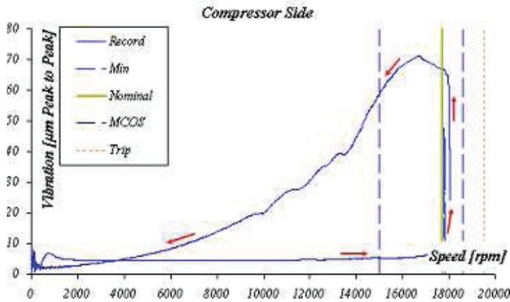
Fig. 4. Vibration hysteresis in Bode plot. Typical behavior for a spiral vibration [1]
