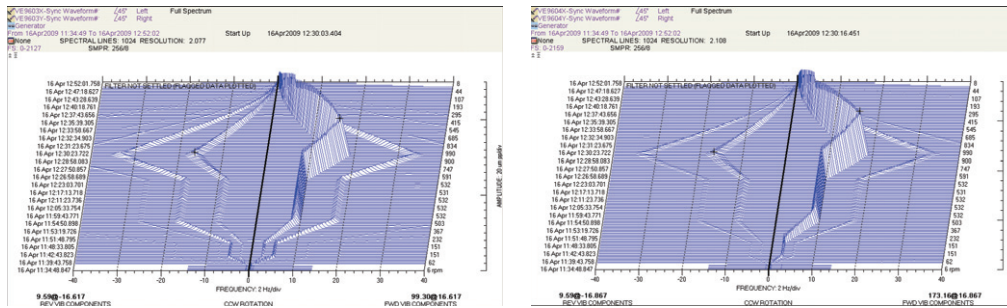
Fig. 8. Full Waterfall plot of DE and NDE generator bearings showing dominant 1X forward vibration component (circular orbit)
