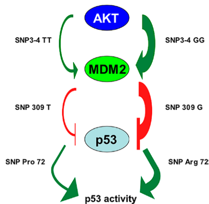
Figure 4. Heterogeneity of the p53 Pathway
