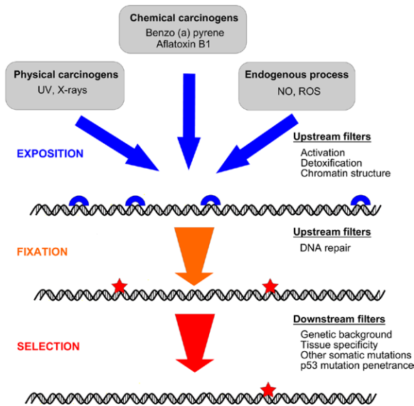
Figure 1. Shaping p53 Mutations in Human Cancer
