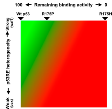
Figure 2. Heterogeneity of the DNA-Binding Activity of Mutant p53
