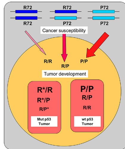
Figure 3. Complexity of p53 R72P Polymorphism
