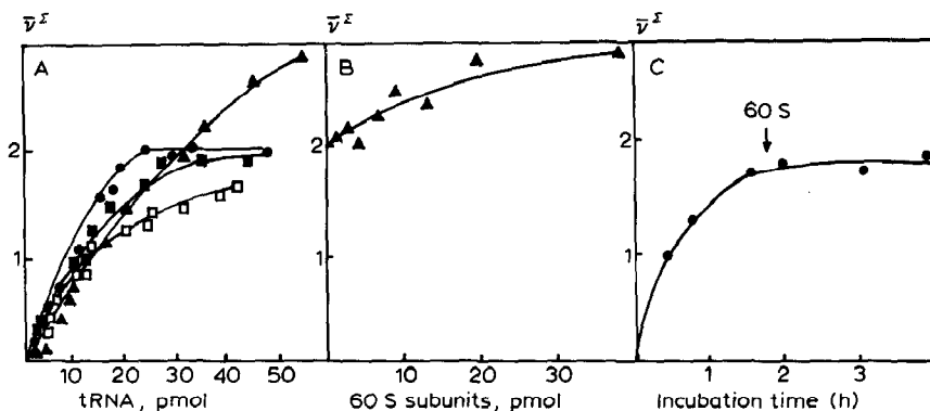
Fig.2. (A) Titration of 80 S ribosomes with different tRNA Phe forms. The incubation mixture contained in 50 \mu l of buffer TAM, 10 pmol 80 S ribosomes, 6 \mu g poly(U) and increasing amounts of [ 14 C]Phe-tRNA Phe (■), Ac[ 14 C]Phe-tRNA Phe (●) or [ 14 C]tRNA Phe (▲). Ac[ 14 C]Phe-tRNA Phe binding at 10 mM Mg 2+ (□). The incubation was for 60 min at 0°C. (B) Effect of 60 S subunit on E site formation. The mixture contained 10 pmol 40 S subunits, 6 \mu g poly(U) and 64 pmol [ 14 C]tRNA Phe in 50 \mu l of buffer TAM. After incubation for 90 min at 0°C the increasing amounts of 60 S subunits were added and the samples were incubated for the next 60 min. (C) Kinetics of Ac[ 14 C]Phe-tRNA Phe binding to ribosome. The mixture contained 10 pmol 40 S subunits, 4 \mu g poly(U) and 98 pmol Ac[ 14 C]Phe-tRNA Phe in 20 \mu l of buffer TAM. After 100 min of incubation at 0°C 20 pmol, the 60 S subunits were added to 30 \mu l and kinetic measurements were continued.
