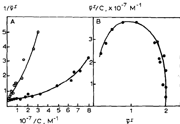
Fig.3. Titration curves of Ac[ 14 C]Phe-tRNA Phe binding to ribosomes. (A) Double reciprocal plots at 20 mM Mg 2+ (●) and 10 mM Mg 2+ (○). (B) Scatchard plots at 20 mM Mg 2+ . The experimental data are from fig.2A.
