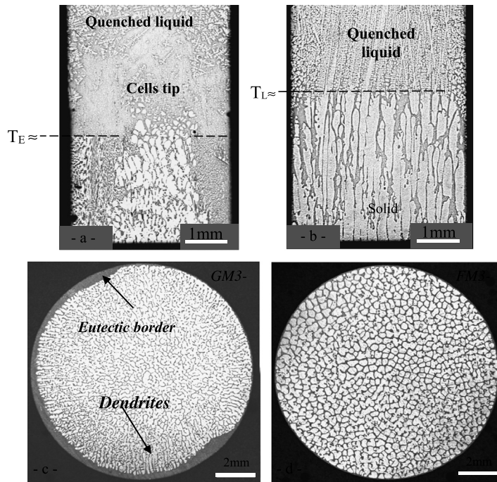
Fig. 6. Comparison of the microstructures obtained during upward solidification on ground (a and c) and in microgravity (b and d) for Al-1.5wt%Ni, G = 24 K/cm and V = 2.3 \mu\text{m/s} . (a) and (b): Longitudinal sections across the quenched front, (c) and (d) transverse sections below the quenched front.
