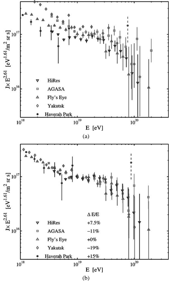
Fig. 1. Currently available data on the highest energy cosmic rays. The quantity J is the differential energy flux, d\phi/dE , per unit time per unit area per steradian. Panel (a) shows the data as published by the five experimental collaborations: AGASA [1], Fly’s Eye [2], Haverah Park [3], HiRes [4], and Yakutsk [5]. Panel (b) shows the data after adjusting the absolute energy calibrations of the various experiments so as to bring the results from the different experiments into agreement at 10^{19} eV. For specificity, the Fly’s Eye absolute energy scale was adopted as the standard. The fractional shifts in absolute energy scale, \Delta E/E , shown in the figure, are all well within the published systematic errors in the energy scale.
