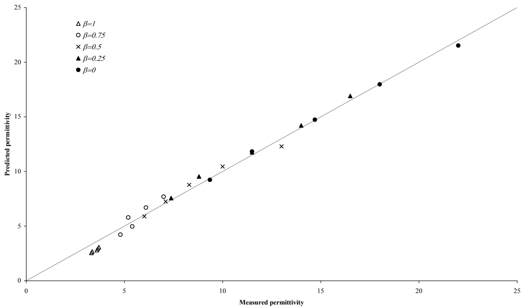
Figure 4 Relationship between calculated and measured dielectric permittivity ( \epsilon'_{sw-NAPL} ) at different \beta values.
