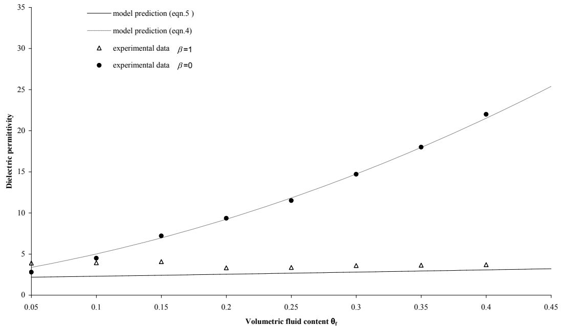
Figure 2 Effect of volumetric fluid content ( \theta_f ) on dielectric permittivity of soil-water ( \varepsilon'_{sw} ) and soil-water-NAPL ( \varepsilon'_{sNAPL} ) mixtures.
