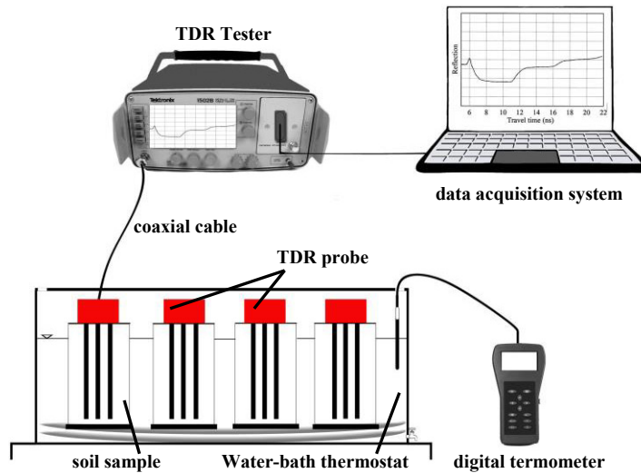
Figure 1 Experimental setup used in the experiment.
