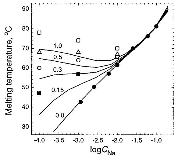
FIGURE 7 Comparison of experimental (points) (Record, 1975) and calculated PB theory (curves) values of T_m dependence on Na^+ concentration for different values of r = C_{Mg}/C_p (indicated near the corresponding theoretical curves). Experimental points are marked for different r as follows: 0.0 (●), T_m values were used in calculation of \Delta G^{mel} , 0.15 (■), 0.3 (○), 0.5 (△), 1.0 (□). The parameters used in the calculations are C_p = 0.042 mM, b_h = 1.69 Å, a_h = 9.5 Å, b_c = 3.38 Å, a_c = 7.0 Å, d_{Na} = d_{Cl} = 2 Å, d_{Mg} = 3 Å.
