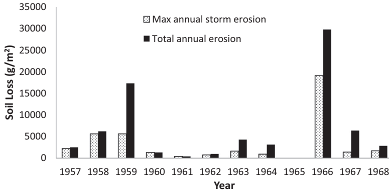
Fig. 10. Soil loss in the maximum annual erosion event and annual total soil loss on the cropland plot.
