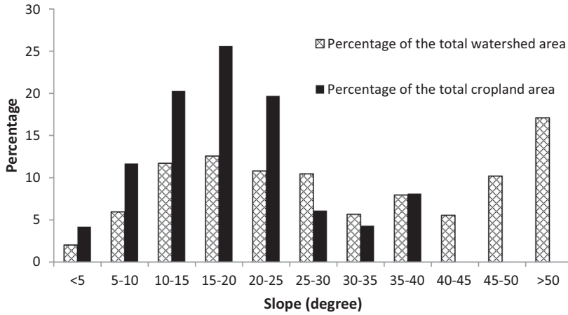
Fig. 2. Slope classification of watershed and cropland in Wangjiagou.
