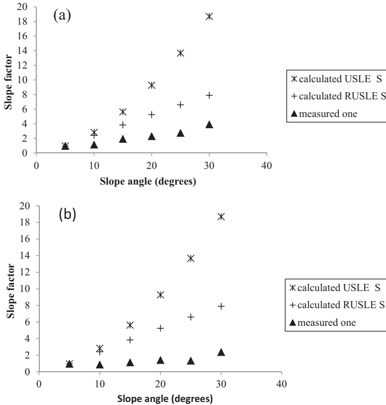
Fig. 7. Comparison of calculated S factors and measured ones (a) Short Slope (SSP) and (b) Long Slope (LSP) plots.
