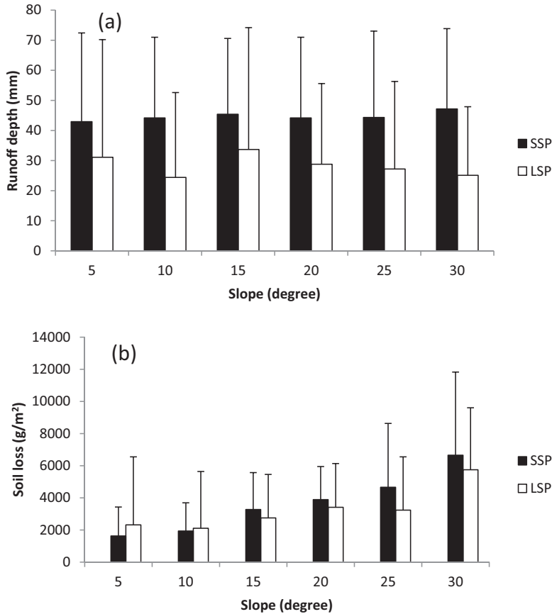
Fig. 6. Mean annual runoff and soil loss on Short Slope (SSP) and Long Slope (LSP) plots and their standard deviation error bars: (a) runoff and (b) soil loss.
