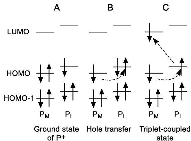
Fig. 9. Schematic of electronic transitions affecting P + .
