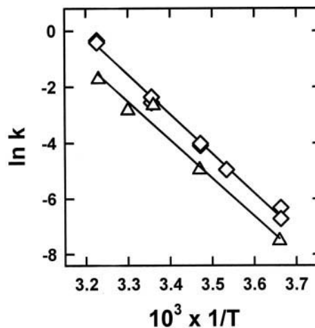
FIGURE 5 Arrhenius plot. Upper curve ( \diamond ), high concentration of reactants: donor ( 100\ \mu\text{l} labeled red cells) plus acceptor (72 mg MBCD/3.9 mg cholesterol) in 1 ml final volume. Lower curve ( \triangle ), low concentration of reactants: donor ( 100\ \mu\text{l} red cells) plus acceptor (19 mg MBCD bearing 1 mg cholesterol) in 10 ml final volume. Reactions were carried out between 0 and 37^\circ\text{C} as in Fig. 1. Time courses were fit to a first-order exponential expression and the derived kinetic constants plotted against inverse temperature. Energies of activation were estimated from the Arrhenius expression, \ln k = E_{\text{act}}/RT .
