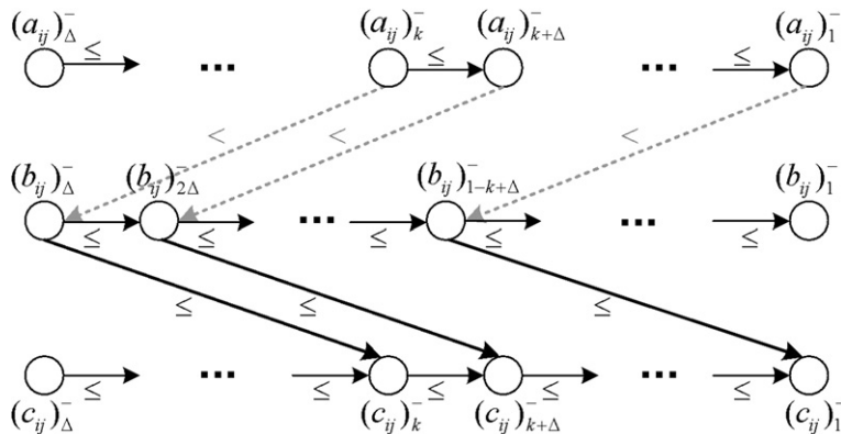
Fig. 8. Linear constraints (73)–(74).
