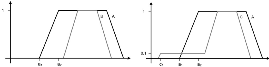
Fig. 3. Since the definition of the fuzzy time intervals B and C are similar, it is desirable that |bb_d^{\leftarrow}(A, B) - bb_d^{\leftarrow}(A, C)| is small.
