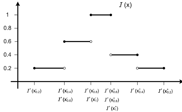
Fig. 6. There exists an FI_M -interpretation \mathcal{I} for a set of FI-formulas \Theta iff there exists a P-interpretation \mathcal{I}' for the corresponding set \Psi of linear constraints.
