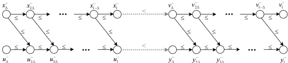
Fig. 11. Linear constraints (93)–(95).
