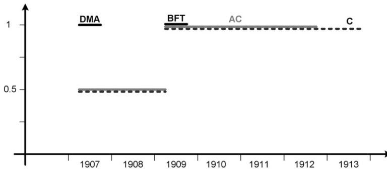
Fig. 7. FI-interpretation of events corresponding to the creation of Bread and Fruit Dish on a Table ( BFT ) and the Demoiselles d’Avignon ( DMA ), as well as Picasso’s Analytical Cubism ( AC ) and Cubism ( C ) periods.
