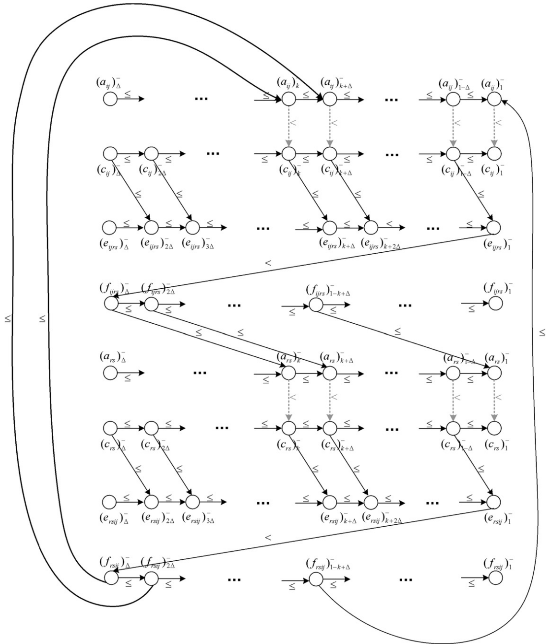
Fig. 10. Linear constraints (84)–(89).
