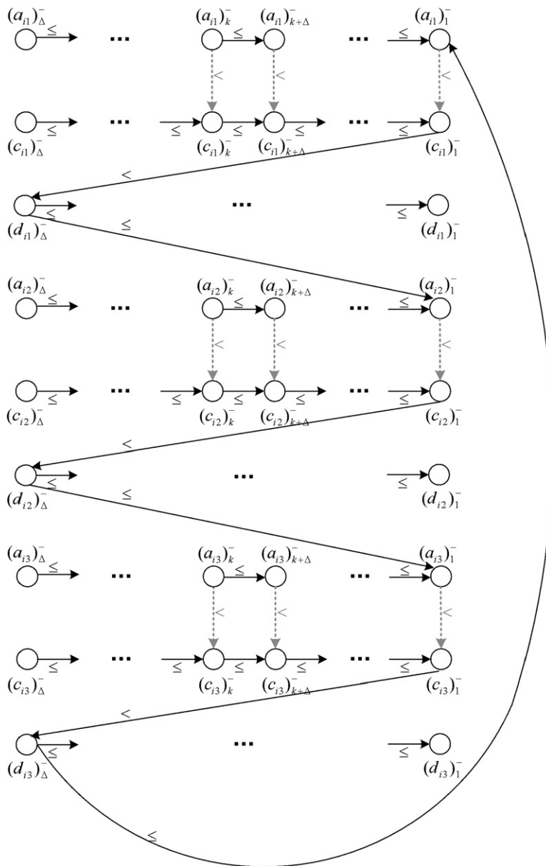
Fig. 9. Linear constraints (75)–(77).
