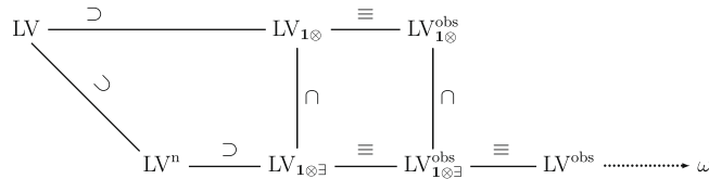
Fig. 1. Linear languages discussed in Section 2 and the road to \omega .
