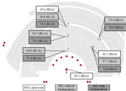
Fig. 1. Overall A-weighted background noise levels and speech sound pressure levels dB(A), unoccupied condition. Sources in red.
