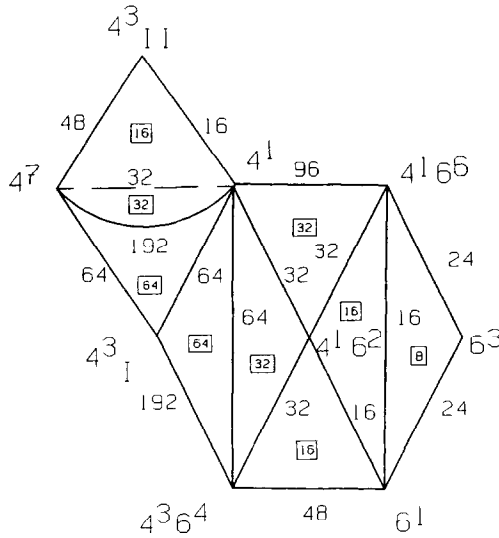
FIG. 1. The quotient of the poset space under the action of M_{12} .
