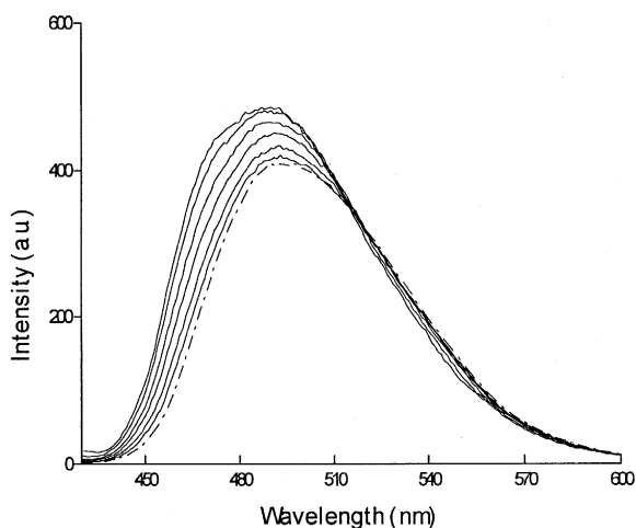
Fig. 2. Fluorescence emission spectra of DIP in aqueous solution pH 7 in the absence (---) and in the presence of DMPC vesicles (—). Concentrations of DMPC are (in order of increasing intensity, in mM): 0.146, 0.239, 0.414, 0.654, 1.16 and 1.96. Concentration of DIP, 1 \times 10^{-5} M; excitation wavelength, 415 nm.
