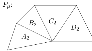
Fig. 4. The sets $A_2, B_2, C_2$ and $D_2$ assigned to $P_\mu$.
