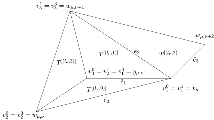
Fig. 5. Notations for the subdivided triangle.
