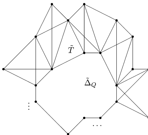
Fig. 9. Construction of the triangulation \Delta_Q .
