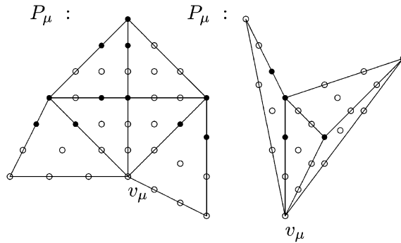
Fig. 8. Admissible sets for S_3^1(\Delta) .
