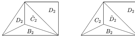
Fig. 6. The sets B_2, \tilde{C}_2, D_2 (resp. B_2, C_2, \tilde{D}_2, D_2 ) assigned to T^{[(l, \nu, \sigma)]} .
