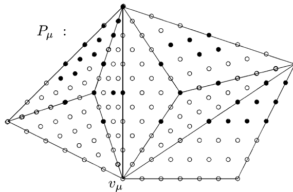
Fig. 11. Admissible sets for S_6^2(\Delta) .
