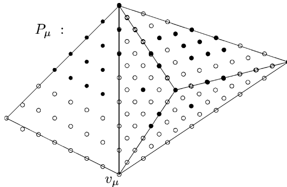
Fig. 10. Admissible sets for S_7^2(\Delta) .
