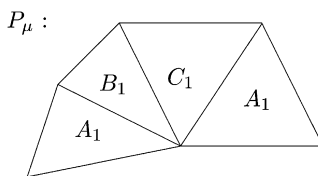
Fig. 3. The sets $A_1$, $B_1$ and $C_1$ assigned to $P_\mu$.
