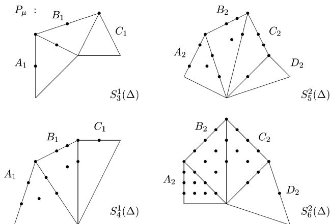
Fig. 7. Lagrange interpolation points.
