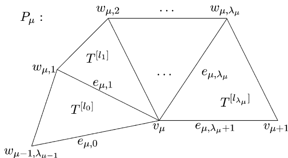
Fig. 1. The polyhedron P_\mu .
