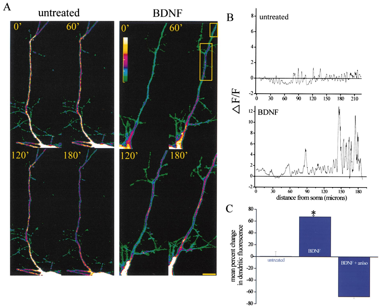
Figure 2. Time-Lapse Imaging of BDNF-Stimulated Translation
