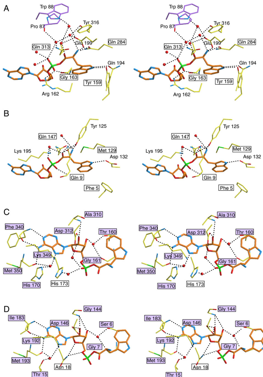
Figure 6. Close-Up Views of the Trp-AMP Binding Site of Human and B. stearothersophilus TrpRSs
