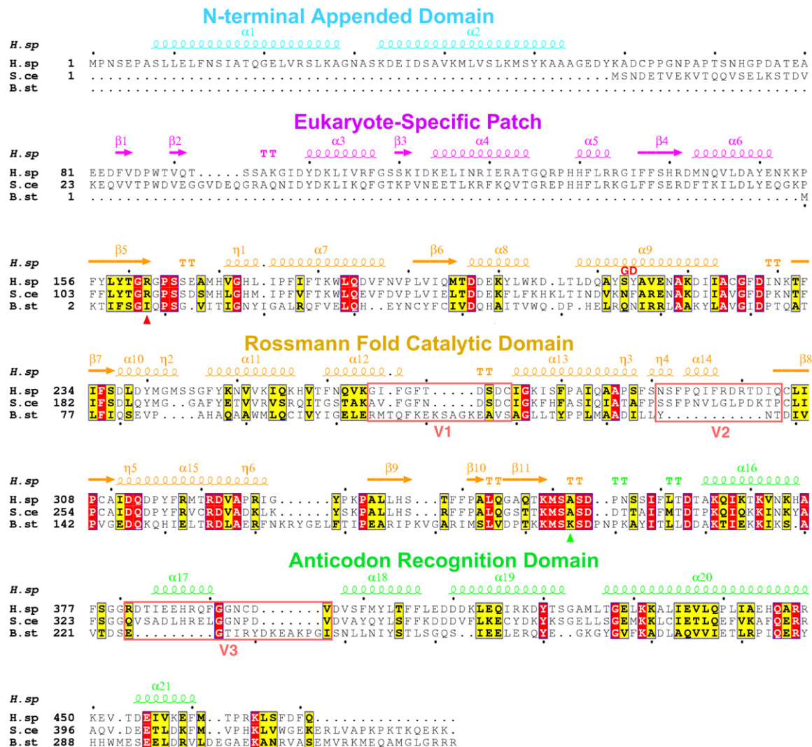
Figure 5. Structural Alignment of Human and B. stearothersophilus TrpRSs
