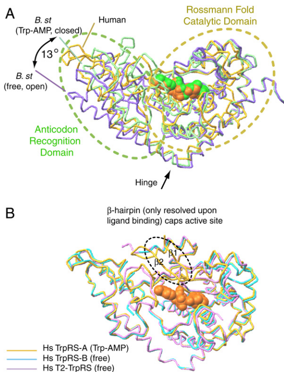
Figure 7. Human and B. stearotherophilus TrpRSs Use a Distinct Mechanism to Close the Active Site for Catalysis
