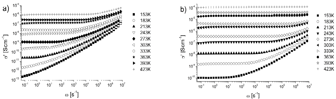
Fig. 5. Real part of conductivity versus frequency measured at different temperatures for (a) 40BaO–60V 2 O 5 and (b) 30BaO–70V 2 O 5 (in %mol) glass samples.
