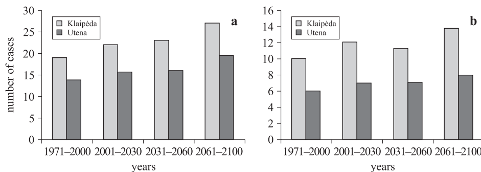
Figure 8. Dynamics of the number of cases (per year) when daily precipitation exceeds 10 mm (a) and 3-day precipitation exceeds 20 mm (b) for the 21st century, simulated by CCLM model output data according to the A1B emission scenario
