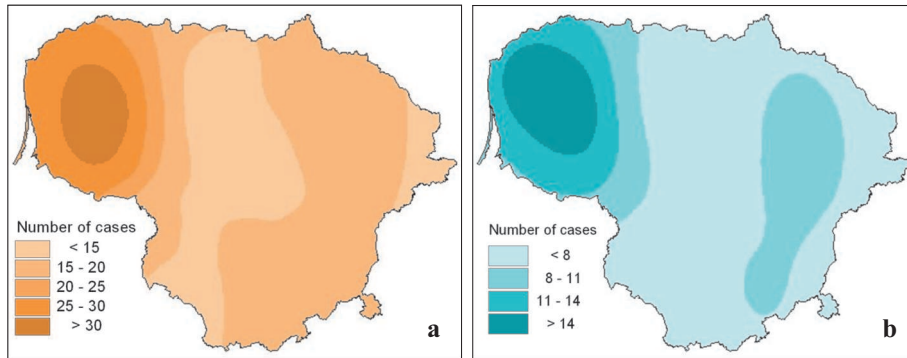
Figure 9. The number of cases with daily precipitation exceeding 10 mm (a) and 3-day precipitation exceeding 20 mm (b) for the year 2100, simulated using CCLM model output data according to the A1B emission scenario
