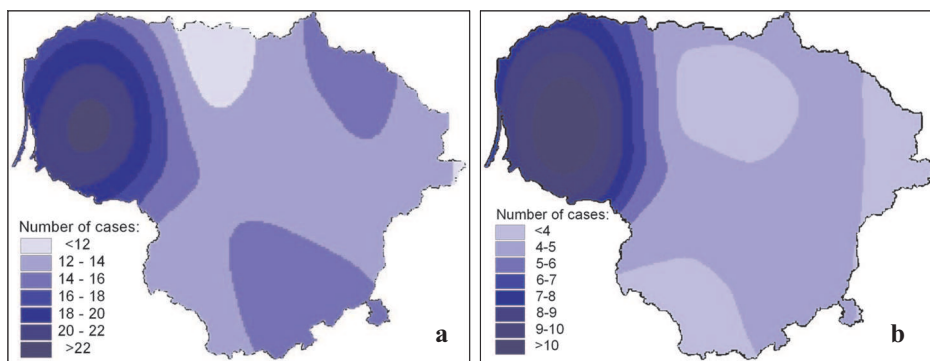
Figure 3. Mean number of cases when daily precipitation exceeded 10 mm (a) and 3-day precipitation exceeded 20 mm (b) in Lithuania in 1961–2008
