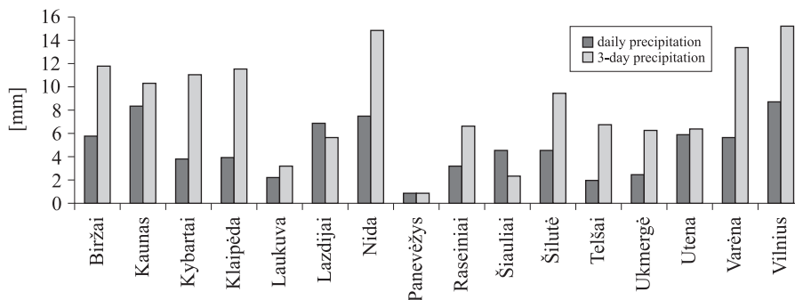
Figure 7. Mean annual daily and 3-day maxima of precipitation differences between two periods (1985–2008 average minus the 1961–1984 average) at 16 meteorological stations in Lithuania. Positive changes show a precipitation increase
