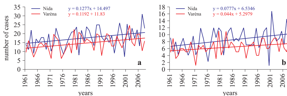
Figure 6. Changes in the number of heavy precipitation events (> 10 mm daily precipitation (a) and 20 mm 3-day precipitation (b)) at Nida and Varėna in 1961–2008. All trends are statistically significant according to the Mann-Kendall test
