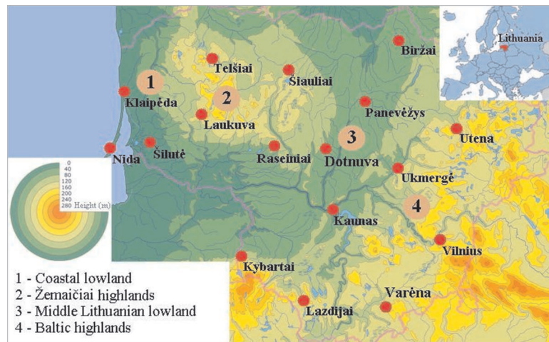
Figure 1. Locations of the meteorological stations from which data were used in the study
