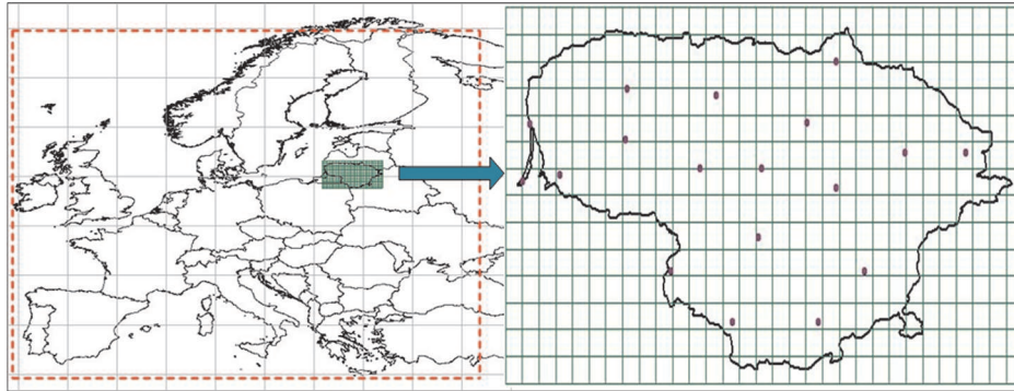
Figure 2. The CCLM model domain covering Lithuanian territory (dotted line on the left) and the regular grid (spatial resolution 0.2^\circ ) over the country (on the right). The black dots represent the meteorological stations from which data were used in this research
