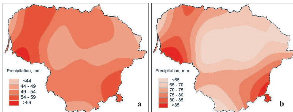
Figure 4. Ten-year return level of the daily (a) and 3-day (b) precipitation [mm] maximum in Lithuania
