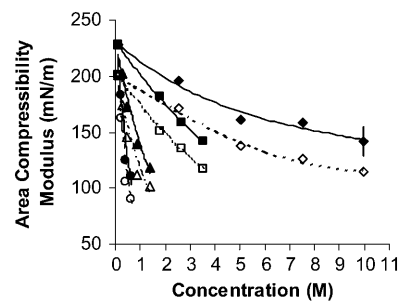
FIGURE 5 Average area compressibility modulus, K_A (solid marks) and K_{app} (open marks), of SOPC vesicles in alcohol/water mixtures. Symbols are methanol (diamonds), ethanol (squares), propanol (triangles), and butanol (circles). Bar indicates 1 SD. For clarity, only one representative error bar of all the measurements is shown (all error bars were equal or less than this one). Differences between control and alcohol-exposed vesicles were statistically significant ( P < 0.05 ) as evaluated by Student's t -test ( \alpha = 0.05 ).
