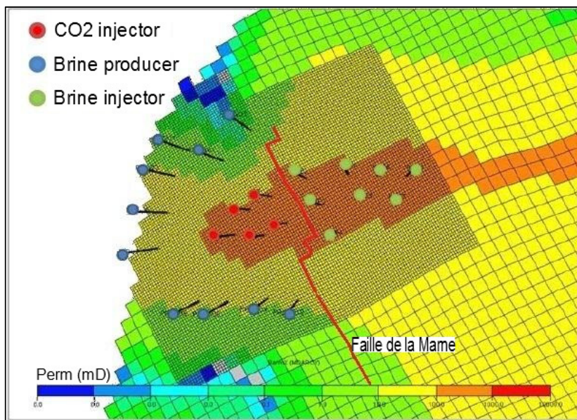
Fig. 5- Site model of Buntsandstein site with grid refinement. Wells configuration as for the injection west of the Marne Fault (“Faille de la Marne” represented by the red line).
