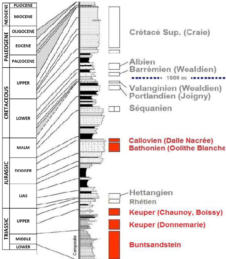
Fig. 1- Selection of the stratigraphic target suitable for CO 2 storage. Buntsandstein sandstones, Donnemarie, Chaunoy and Boissy sandstones (Keuper) and Dogger limestones. These targets are represented on the Paris Basin log (modified from Guillocheau et al., 2000 [8]).
