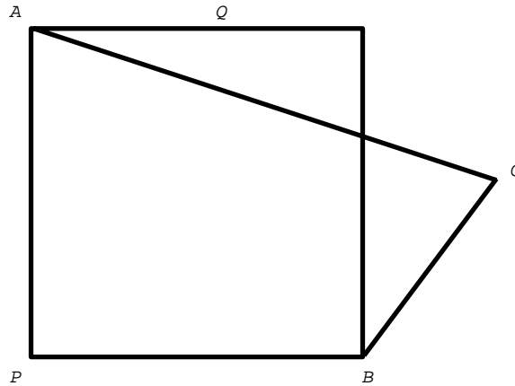
Fig. 14. Construction of a functional linkage for the complex conjugation.
