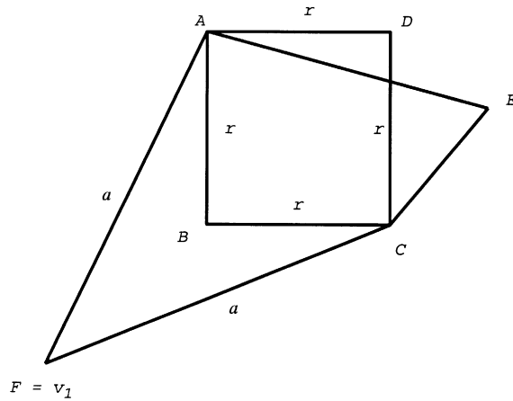
Fig. 11. The modified Peaucellier invensor \mathcal{J}_t : the square ABCD is rigidified and \ell[AE] - \ell[EC] = 2\varepsilon > 0 , \ell[EC] > r .
