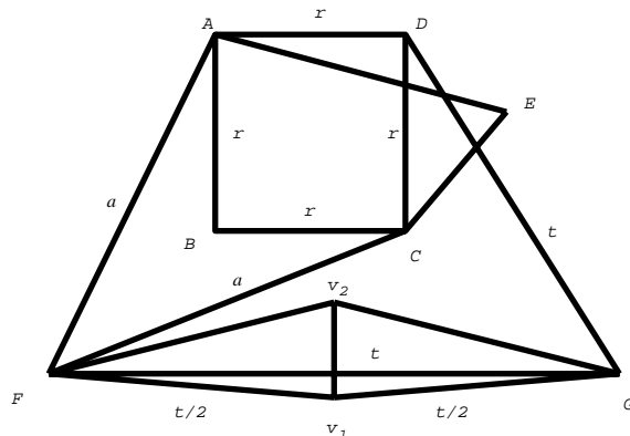
Fig. 13. The based Peaucellier straight-line motion linkage \tilde{\mathcal{S}} : \ell[v_1 v_2]^2 + (t/2)^2 = \ell[Fv_2]^2 = \ell[Gv_2]^2 . The image of B under all realizations lies on a segment of the real axis which contains the open interval (-\sqrt{3}/2)t, (\sqrt{3}/2)t \subset \text{Dom}^*(\tilde{\mathcal{S}}) .
