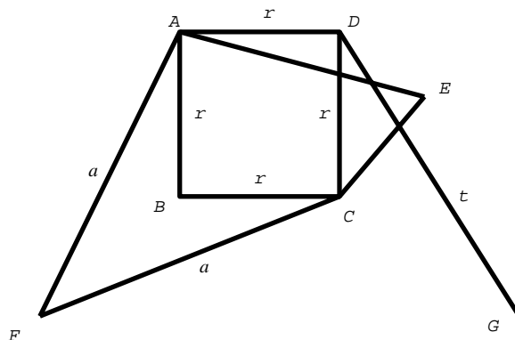
Fig. 12. The Peaucellier straight-line motion linkage \mathcal{S} . The vertices F, G are fixed. The vertex B is the input and output.
