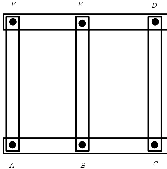
Fig. 5. A mechanical model for the rigidified parallelogram \Sigma .
