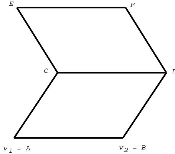
Fig. 7. A translator. The parallelograms \square(ACDB) and \square(CEFD) are rigidified. The set of input/output vertices is \{E, F\} and s = \ell[AC] > t = \ell[CE] .
