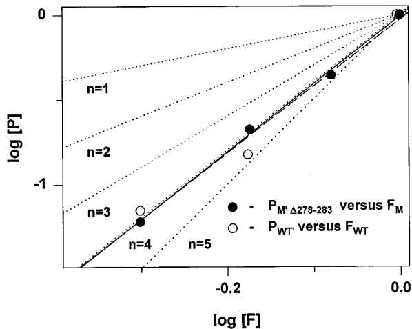
FIGURE 4 Statistical distribution of the single \alpha -rENaC composed from the WT and amiloride-binding domain deletion mutant. Channel reconstitution, recording conditions, treatment of single-channel data, and distinction between channel types were the same as described in Fig. 3. The minimal number of separate observations that represent the fraction of channels in a double-logarithmic plot of statistical distribution of channel types at different \alpha_{WT}:\alpha_{\Delta 278-283} ratios was four for the type WT' and five for the type M', of the respective total number of successful incorporations of channels with a given composition (see Table 2 for the number of observations of each channel type at a given WT:mutant ratio). The solid line represents a best first-order regression fit of the experimental data for type M' (with a slope of 3.89). The dashed line represents a best first-order regression of the experimental data for type WT' (with a slope of 4.02). Dotted lines shown represent theoretical probabilities of random association of two elements into a homo-N-oligomer when the ratio of these elements, calculated with Eqs. 5 and 6, is varied.
