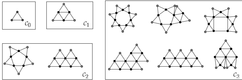
Fig. 1. The classes \mathcal{C}_0, \mathcal{C}_1, \mathcal{C}_2, and \mathcal{C}_3 .
