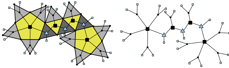
Fig. 3. One element of the family and the associated tree. Dangleings correspond to vertices of type \square .
