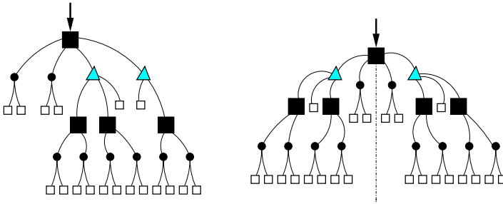
Fig. 4. A ■-mobile and a symmetric ■-mobile.
