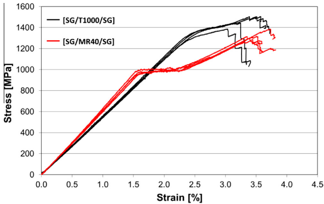
Fig. 6. Tensile stress–strain graphs of S-glass/IM carbon configurations.
