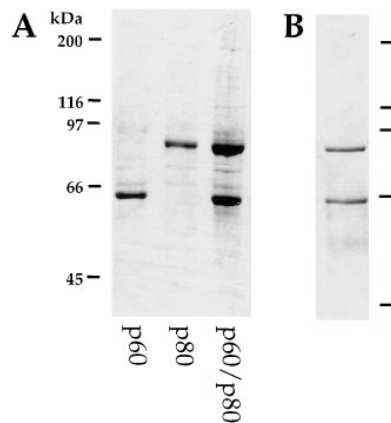
Figure 3. Expression and Purification of Recombinant Katanin Subunits
