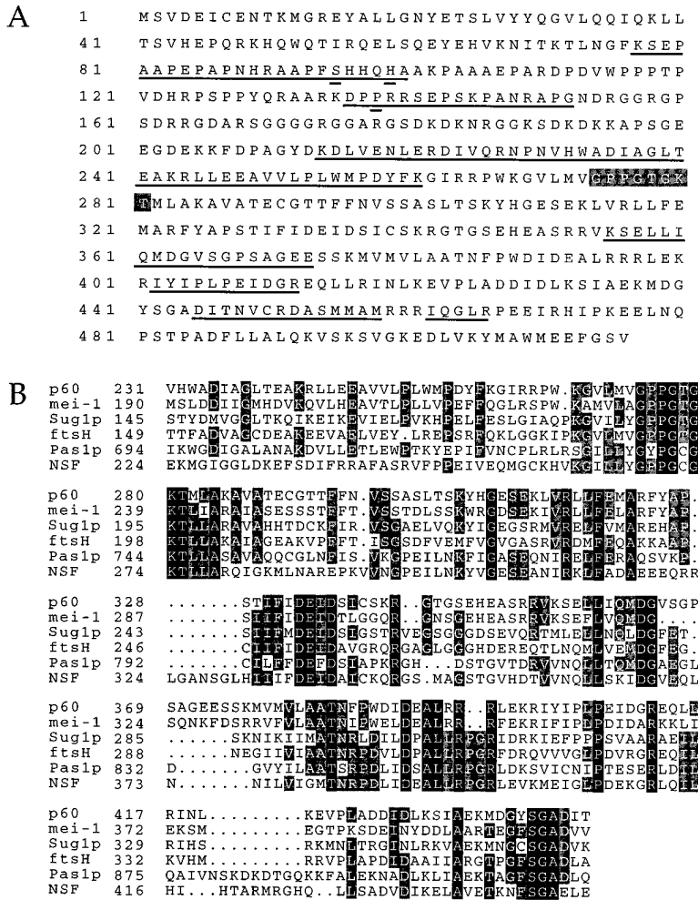
Figure 1. Sequence Analysis of p60 Katanin (A) Predicted protein sequence of the S. purpuratus katanin p60 subunit (GenBank #AF052191). Sequences obtained by direct peptide microsequencing are underlined. Differences between the predicted peptide sequence and that obtained by direct sequencing are indicated by doubled underlines (S95 was reported as F, H99 was reported as P, and P138 was reported as T). The Walker A (P loop) motif is shaded. (B) Amino acid sequence alignment of the p60 AAA domain with AAA members mei-1 ( C. elegans , GenBank #L25423), Sug1p ( S. cerevisiae , GenBank #X66400), ftsH ( E. coli , GenBank #M83138), Pas1p ( S. cerevisiae , GenBank #M58676), and NSF ( C. longicaudatus , GenBank #X15652). Identical residues are shaded black, residues conserved in >60% of the shown members are shaded gray. Left-hand numbering indicates the amino acid residue in the corresponding sequence. Alignment was performed using PILEUP (Genetics Computer Group) and the output was shaded using MACBOXSHADE.
