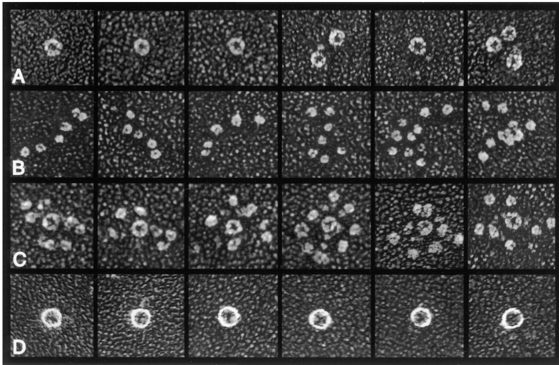
Figure 4. Structure of Katanin as Visualized by Rotary-Shadowing Electron Microscopy
