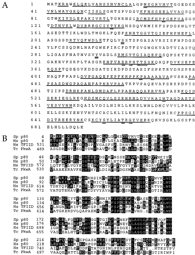
Figure 2. Sequence Analysis of p80 Katanin (A) Predicted protein sequence of the S. purpuratus katanin p80 subunit (GenBank #AF052433). Sequences obtained by direct peptide microsequencing are underlined. Differences between the predicted peptide sequence and that obtained by direct peptide sequencing, or differences found between 2 different p80 cDNA clones are indicated by double underlines. (B) Amino acid sequence alignment of the WD40 repeat region of p80 with a putative human ortholog of p80 (Hs p80, GenBank #AF052432), TFIID ( Homo sapiens , GenBank #U80191), and putative serine/threonine kinase Pkwa ( Thermomonospora curvata , GenBank #P49695). Identical residues are shaded black, residues found in at least 2 sequences are shaded in gray. Left-hand numbering indicates the amino acid residue in the corresponding sequence. Alignment was performed using PILEUP (Genetics Computer Group) and the output was shaded using MACBOXSHADE.
