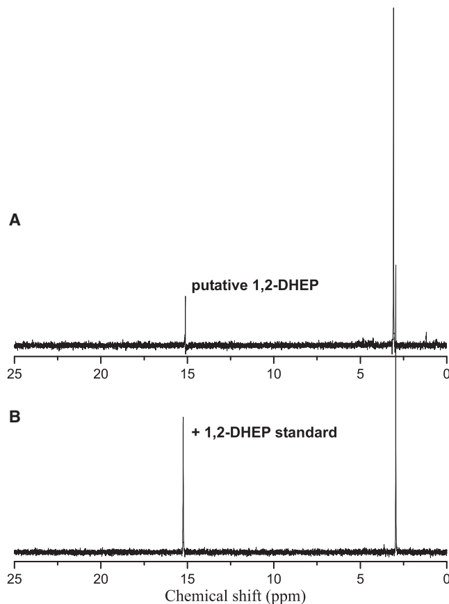
Figure 3. dhpB Mutants Accumulate DHEP
