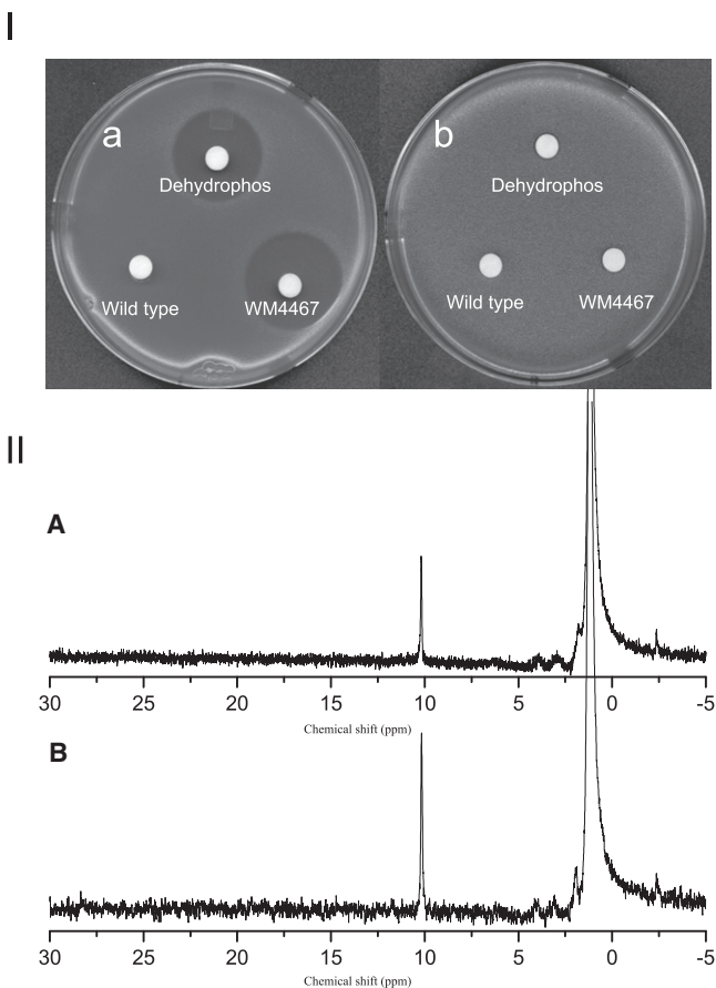
Figure 1. Evidence of Heterologous Production of Dehydrophos in S. lividans
