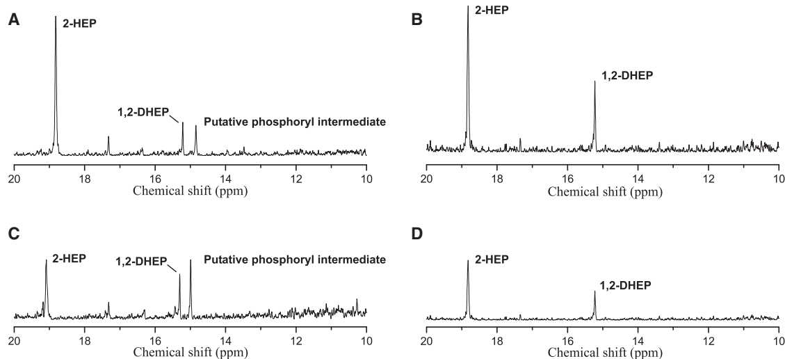
Figure 5. dhpc and dhpH Mutants Accumulate a Phosphate Ester
