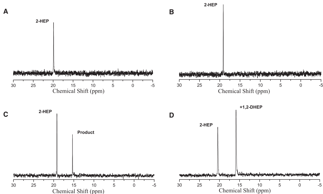
Figure 4. ^{31}\text{P} NMR Spectra of DhpA Assay
