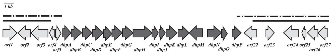
Figure 2. Gene Organization of Fosmid 17E11-4
