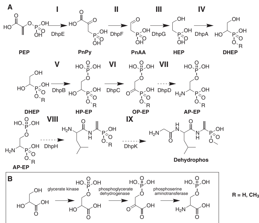
Figure 6. Proposed pathway for dehydrophos biosynthesis (A), and the portion of the serine biosynthetic pathway that bears structural similarity to steps V, VI, and VII of the proposed pathway (B)
