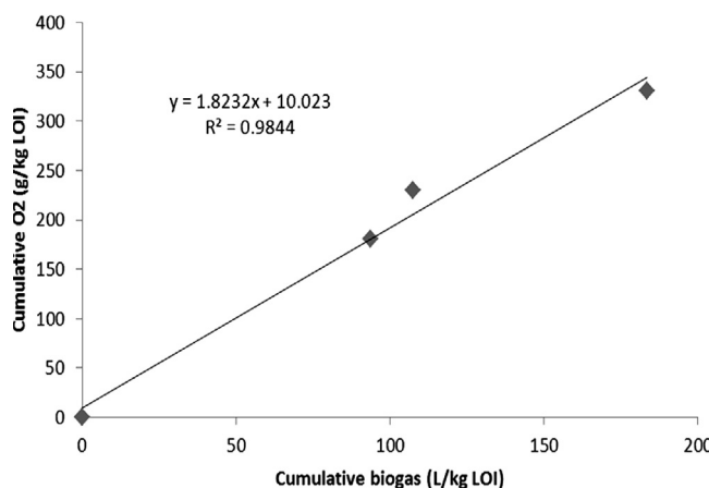
Figure 4 Comparison of final (4 d) production of O 2 test result (g/kg LOI) values to final (116 d) anaerobic biogas test values (cumulative) of three samples (feed; immature compost; mature compost).
