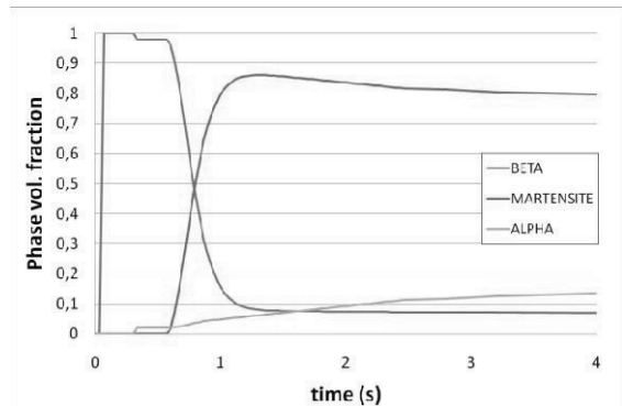
Figure 6. Comparison between the experimentally obtained melted and HAZ and the predicted ones, test 1; (b) phase history of one element of the clad track during the laser cladding of the test 1
