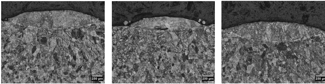
Figure 4. Metallographic picture of the cross sections of the single track samples: (a) 1; (b) 2; (c) 3.
