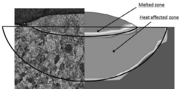
Figure 6. Comparison between the experimentally obtained melted and HAZ and the predicted ones, test 1; (b) phase history of one element of the clad track during the laser cladding of the test 1
