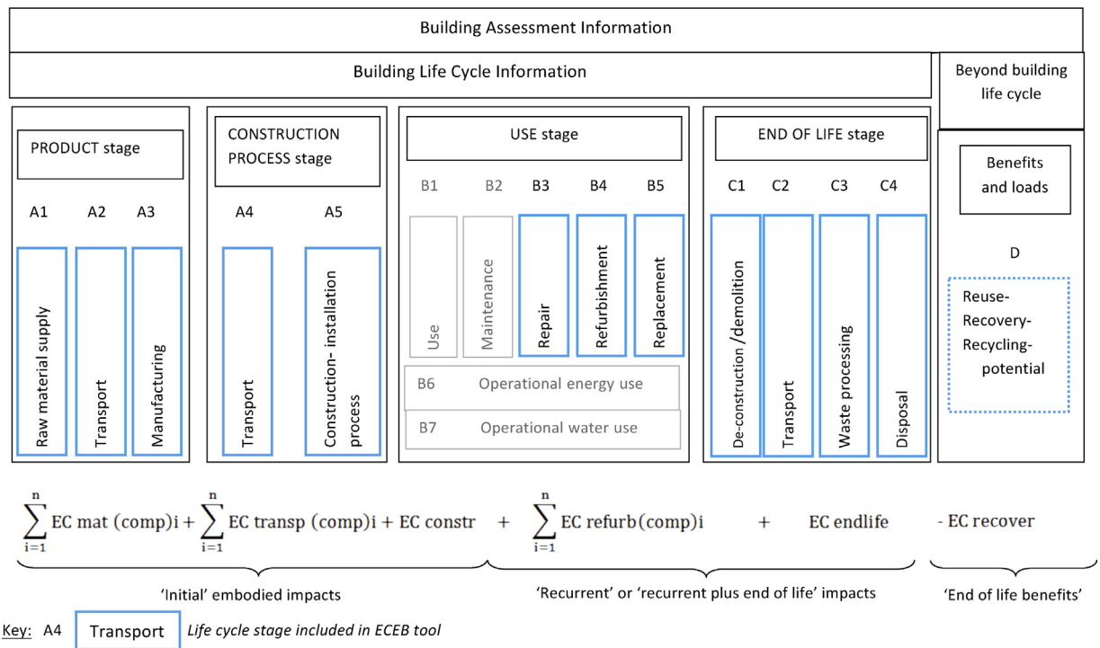
Fig. 1. Life cycle stages from BS EN 15978:2011 Sustainability of construction works – Assessment of environmental performance of buildings – Calculation method [4] mapped against the equation used by the ECEB tool. Key: A4 Life cycle stage included in ECEB tool.
