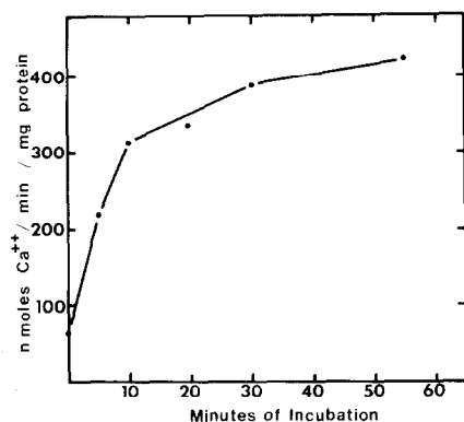
Fig.2. In the presence of 0.68% sodium cholate the \text{Ca}^{++} -ATPase was incubated with phospholipids as described in the legend of fig.1 except that the incubation time was varied as indicated in the figure.
