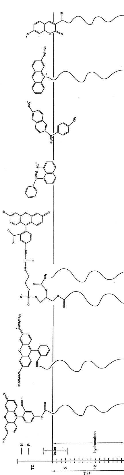
Fig. 4. Schematic figure illustrating the depth of hydrocarbon and acyl linked fluorescent probes. Identity of probes is given in Fig. 1. The location of the phospholipid functional groups is based on the study of Wiener and White [35]. The positions of the nitrobenzyl spin-labels from the bilayer center are shown at the left.
