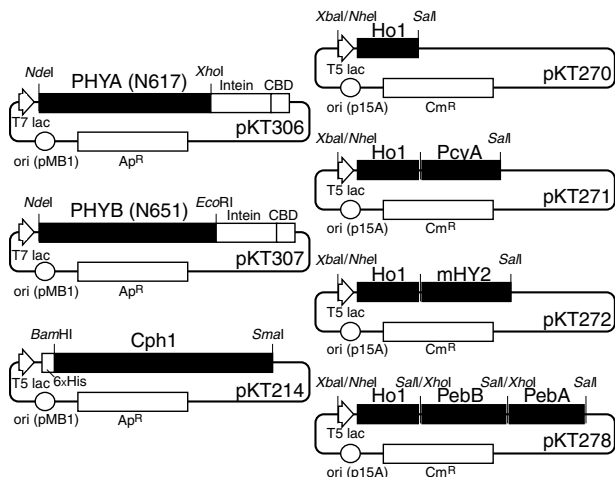
Fig. 1. Plasmid constructs for the expression of phytochrome apoproteins and biosynthesis of various chromophores in E. coli . Plasmids, pKT214, pKT306, and pKT307 are high-copy-number vectors for apophytochrome expression of His-tagged Cph1, chitin-binding-domain (CBD)-tagged PHYA (N617), and CBD-tagged PHYB (N651), respectively. Plasmids, pKT270, pKT271, pKT272, and pKT278 are low-copy-number vectors for the biosynthesis of BV, PCB, PΦB, and PEB, respectively. T5 lac, chimeric promoter for T5 RNA polymerase with the lac operator; T7 lac, T7 promoter with lac operator; Ap R and Cm R , resistance genes for ampicillin and chloramphenicol, respectively; ori (pMB1) and ori (p15A), replication origins from pMB1 and p15A, respectively.
