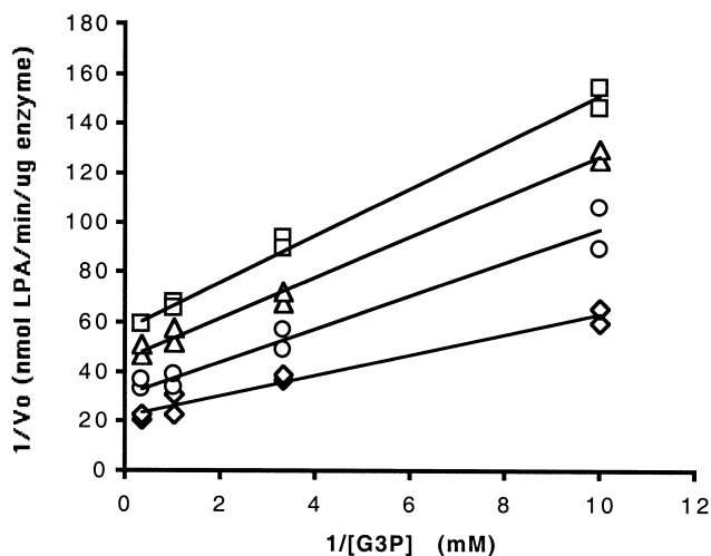
Fig. 1. Determination of squash G3PAT kinetic mechanism. Initial velocity was recorded in assays using varying G3P concentrations at fixed, non-saturating concentrations of acyl-ACP (2 \mu M ( \square ), 3 \mu M ( \Delta ), 5 \mu M ( \circ ), 10 \mu M ( \diamond )). Assays were performed in duplicate. Linear regression shows that the series of lines converge, demonstrating that the enzyme mechanism is sequential rather than substitution.
