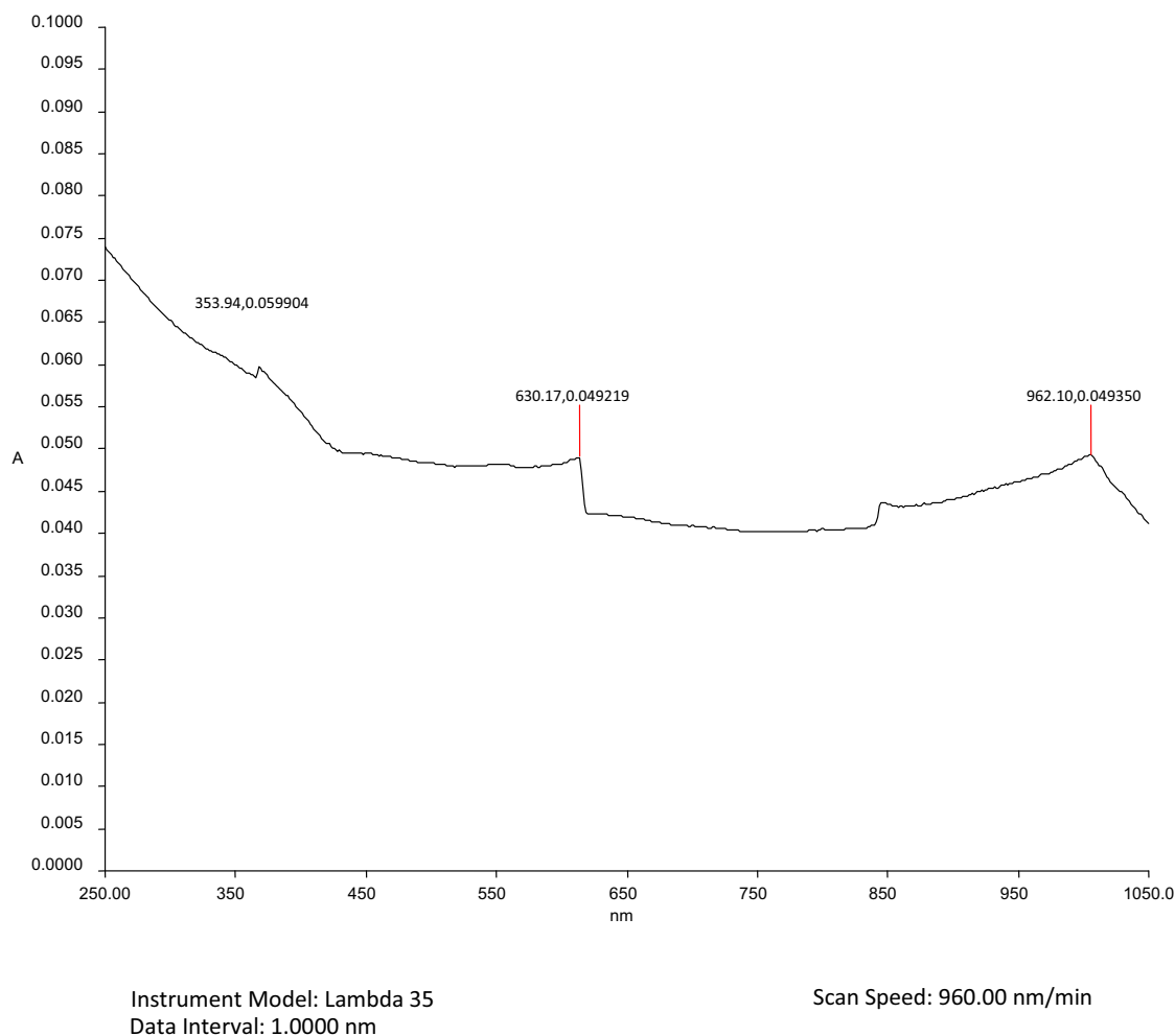
Figure 4 UV-visible spectrum of the [\text{Ni}(\text{C}_{44}\text{H}_{38}\text{N}_6\text{O}_3)\text{Cl}_2] complex.
