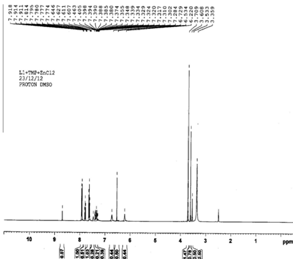
Figure 3 1 H NMR spectrum of the Zn (C 44 H 38 N 6 O 3 ) Cl 2 complex.
