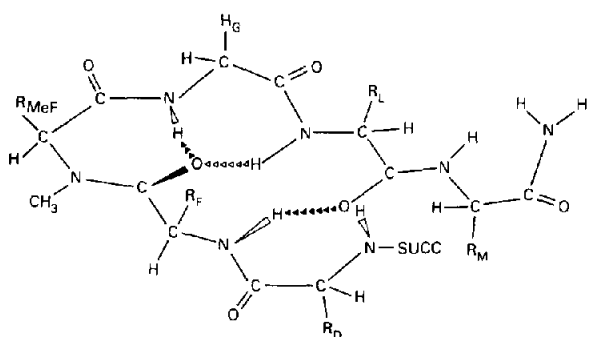
Fig.4. A distorted antiparallel hydrogen bonded (dashed lines) \beta -pleated sheet conformation proposed for senktide. The standard one letter notation for amino acids is used to label the individual residues.
