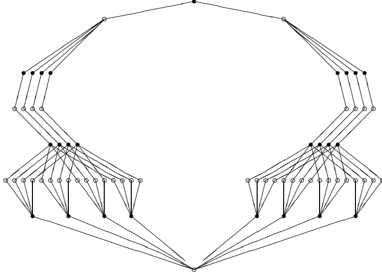
FIGURE 5. P^{III}(2) .
