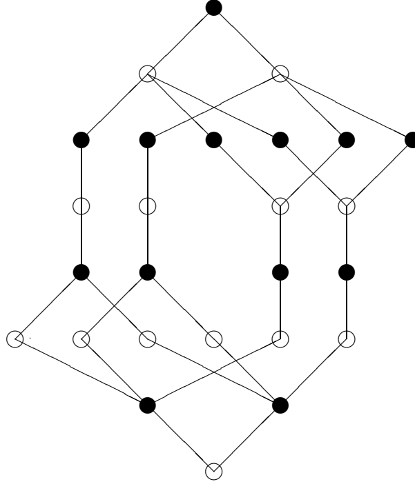
FIGURE 1. P(6, \{[1, 2], [2, 6]\} + \{[2, 5], [5, 6]\}) .
