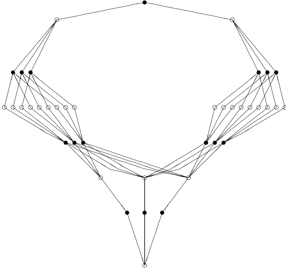
FIGURE 3. P^I(2) .
