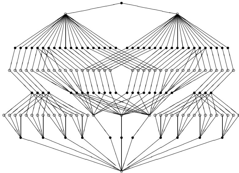
FIGURE 6. P(6, \{[1, 2], [3, 4], [4, 5]\} + \{[3, 5], [5, 6]\} + \{[1, 2], [2, 5]\}) .
