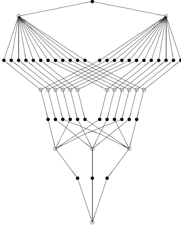
FIGURE 4. P^{II}(2) .
