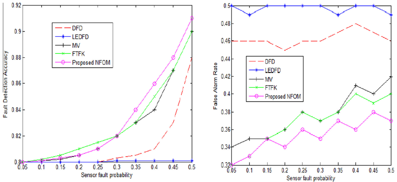
Figure 14 Comparison of FDA and FAR values for random faults with average node density = 10.
