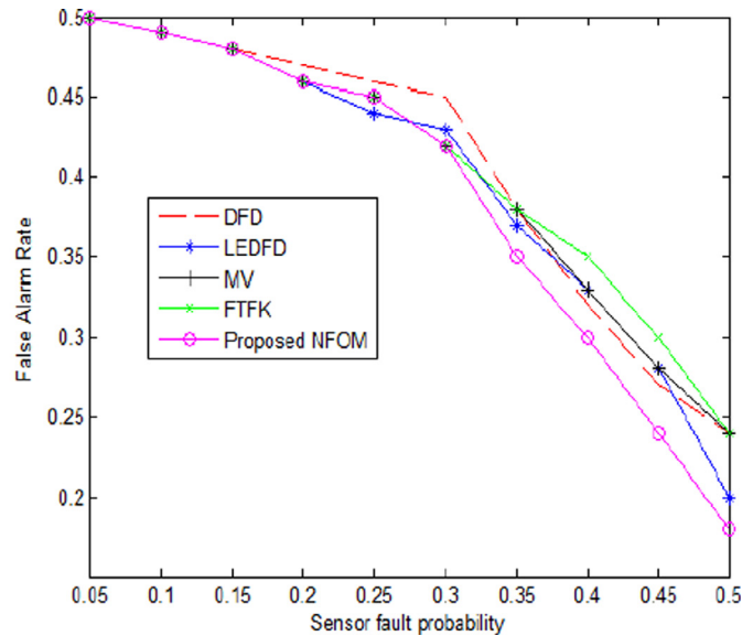
Figure 7 Comparison of FDA and FAR values for fixed faults with average node density = 7.
