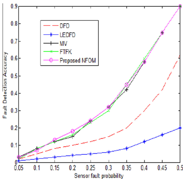
Figure 18 Comparison of FDA and FAR values for mixed faults with average node density = 7.
